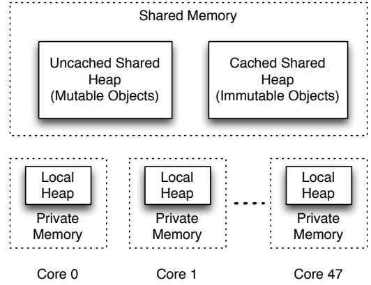
Fig. 1: Heap Layout.
