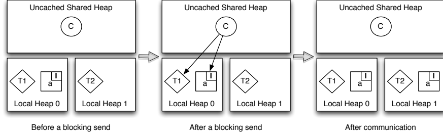
Fig. 5: Steps involved in sending an immutable object a by thread T1 on a shared heap channel C , which is eventually received by thread T2 .
