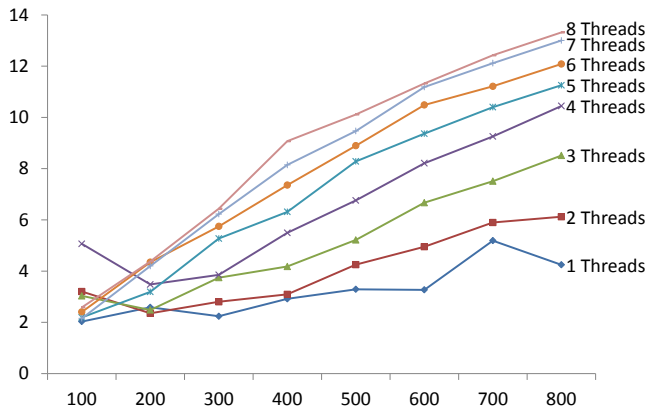
Figure 2. C# GCBench. The x-axis is list problem size, and the y-axis is the slowdown between STM and unsynchronized C# on Bartok. Each line represents a different number of threads.
